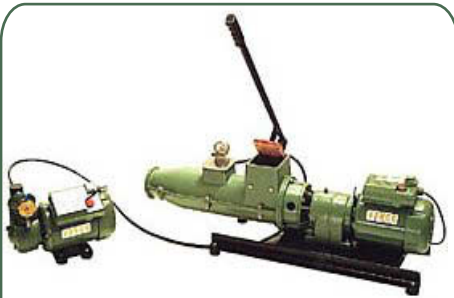
Venco 75mm (3") standard or de-air * the ORIGINAL low cost pugmill which may be easily upgraded to a de-airing unit at a later stage * 400lb/hr output
